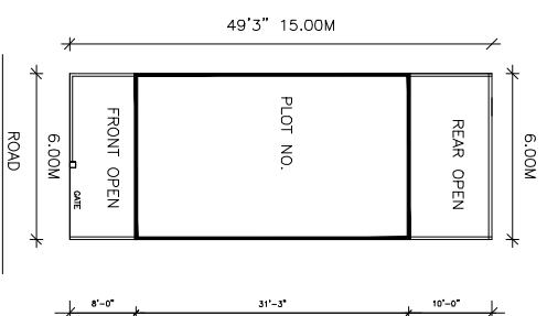
SITE PLAN SCALE 1"=16'
